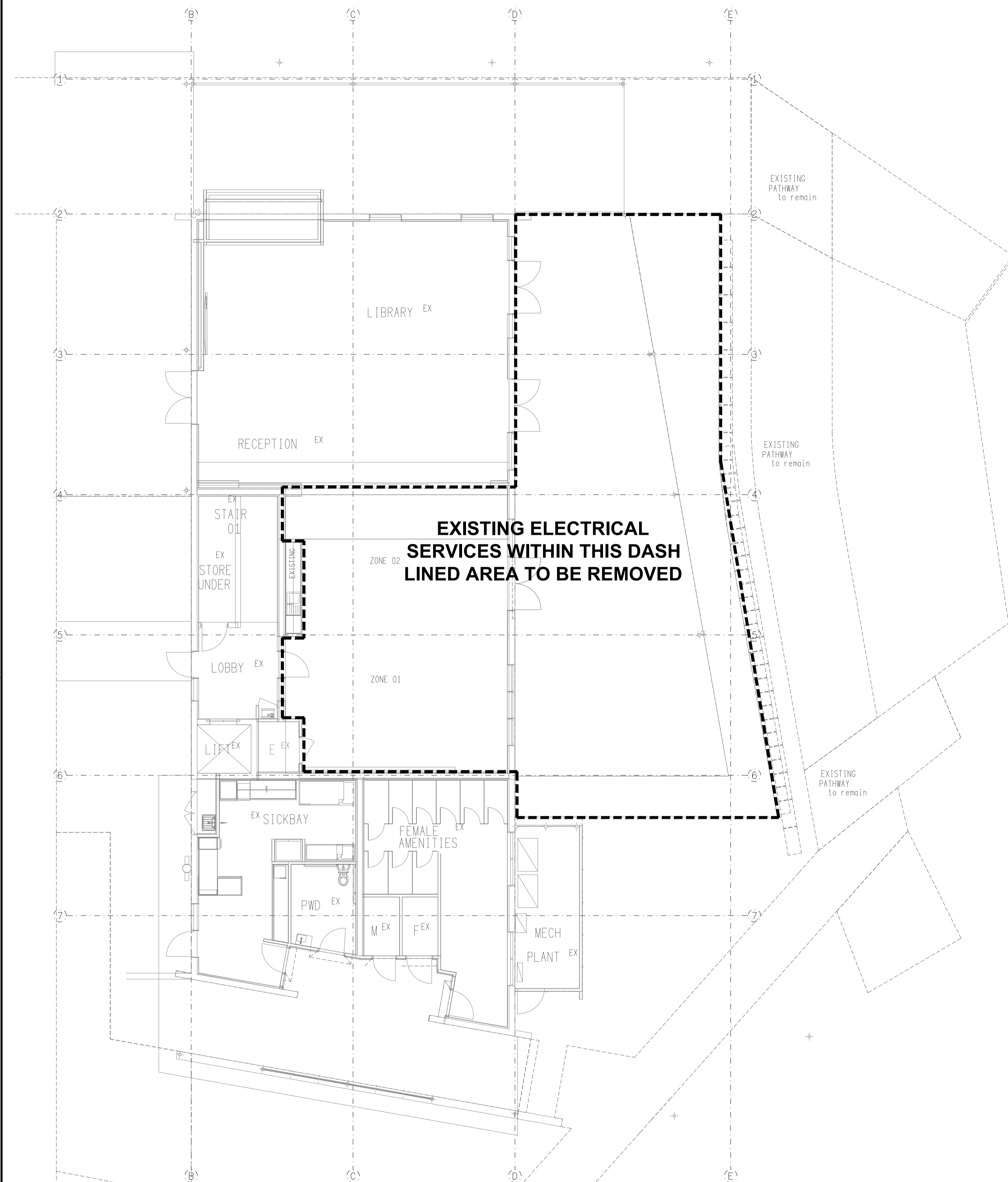
GROUND LEVEL DEMOLITION PLAN SCALE 1:100
